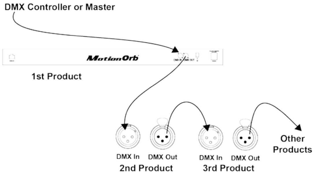
DMX Linking Diagram
